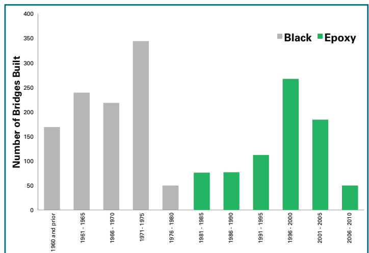
Figure 1: Number of decks used for Markov analysis.
